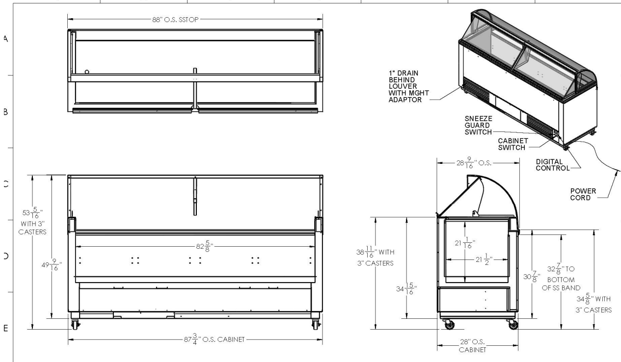
Shown Below Model 16DIPHV-RB
