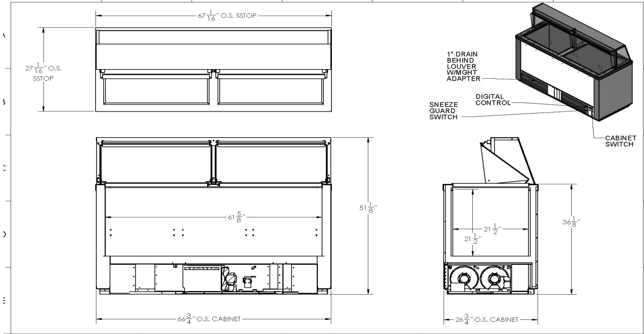
Shown Above: Model 12DIP-RB
