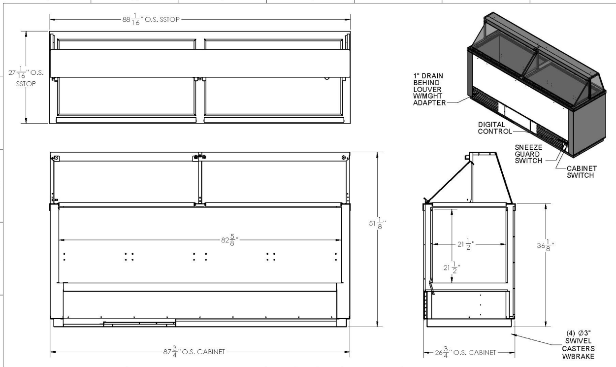
Shown Above: Model 16DIP-RB
