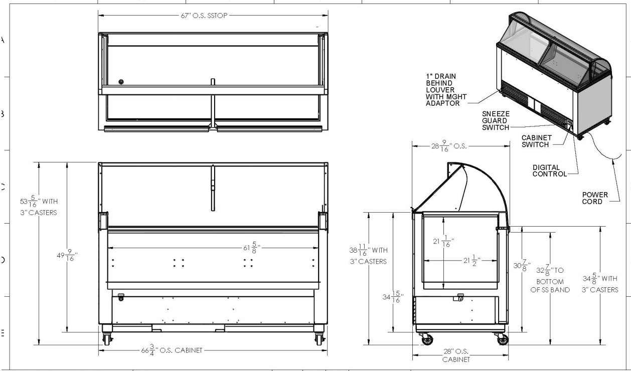
Shown Below Model 12DIPHV-RB
