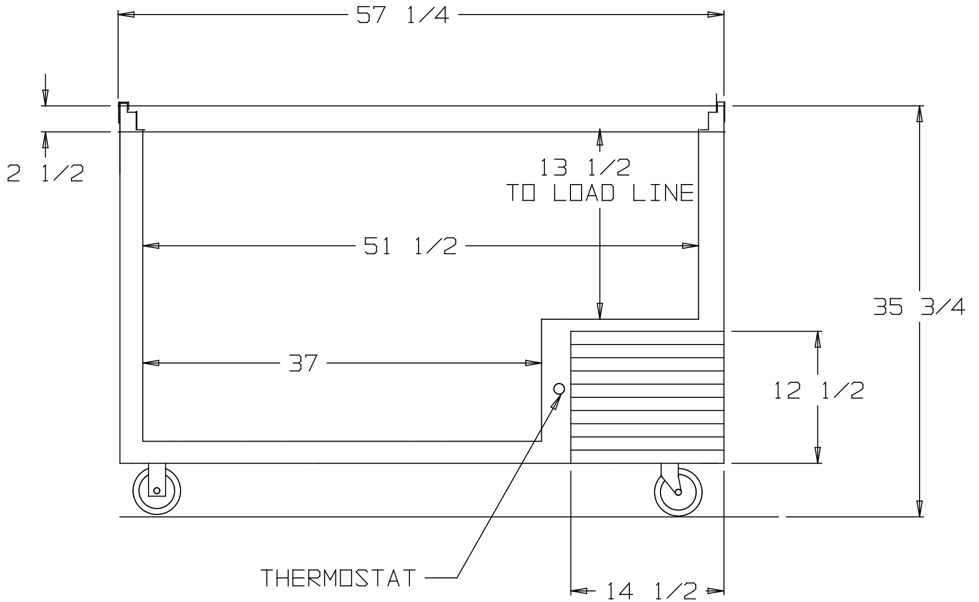
FRONT VIEW CG-15
